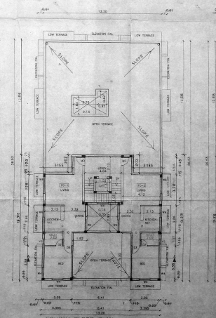
FOURTH FLOOR PLAN
