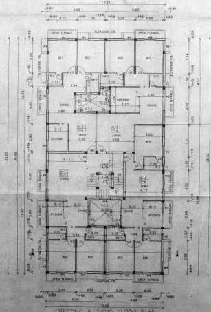
SECOND & THIRD FLOOR PLAN
